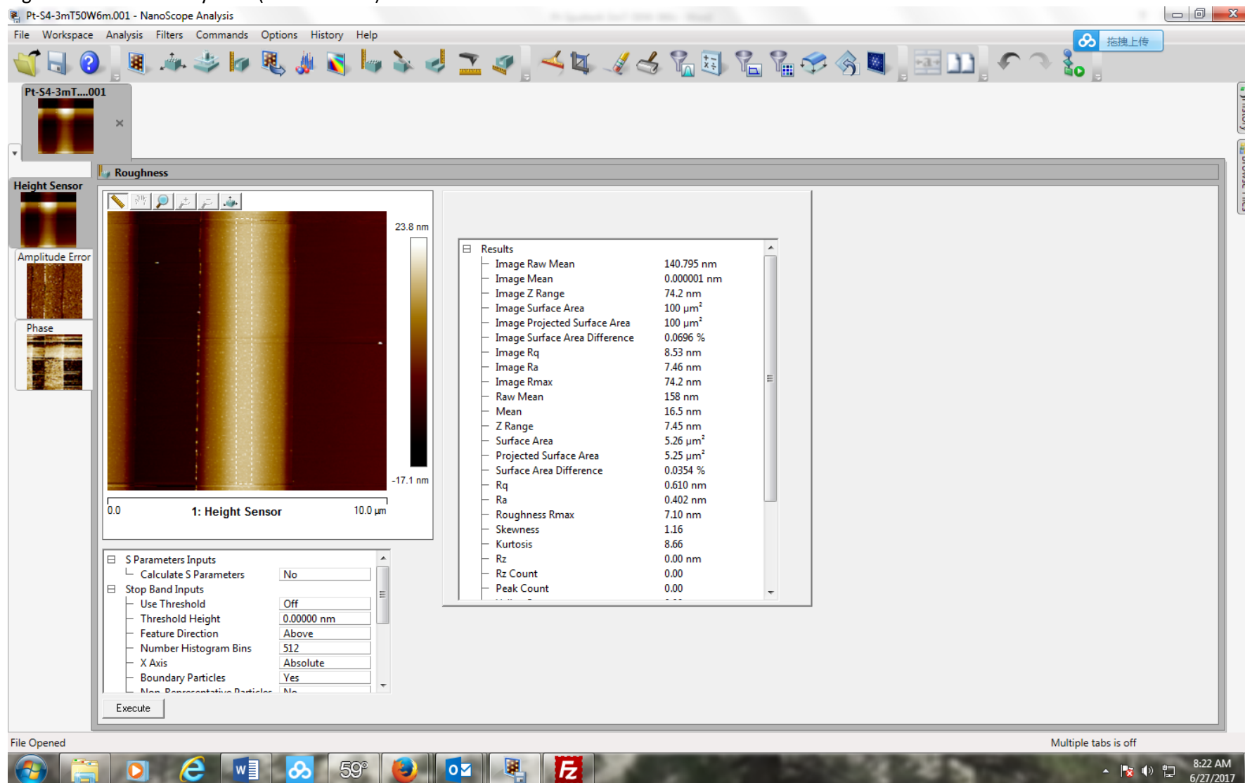
Figure 2 Surface scan by AFM (Ra=0.402 nm).
