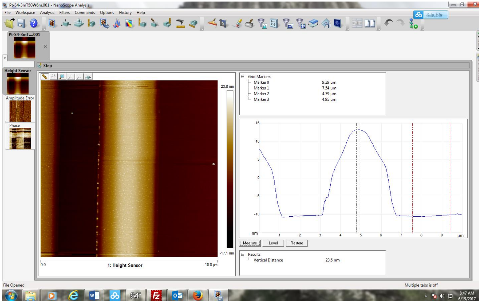
Figure 1 Film Thickness=23.6nm.
